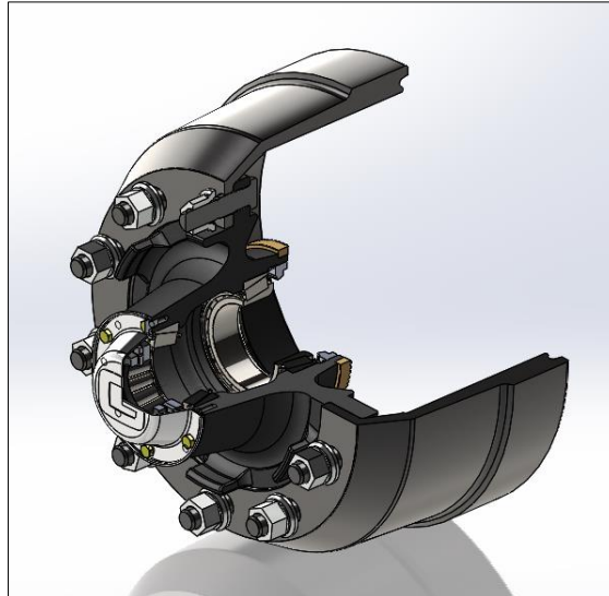
71001A – Single Wheel Stud Hub and Drum Assembly 71001AW – 71001A with 1 x 100 tooth pole wheel 61789
