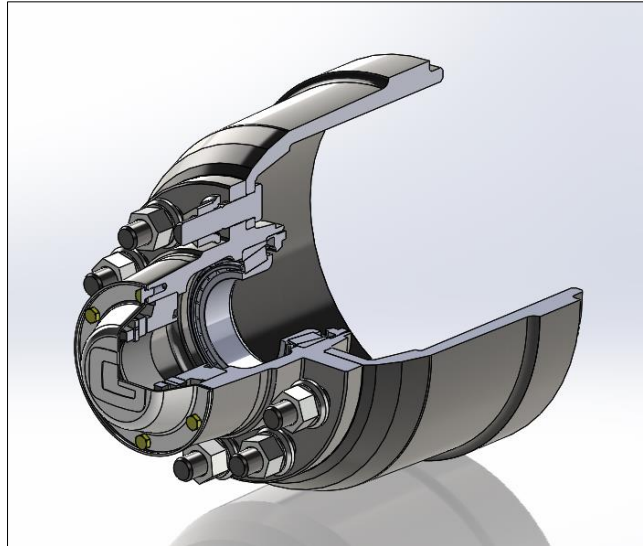
71000A – Twin Wheel Stud Hub and Drum Assembly 71000AW – 71000 with 1 x 80 tooth pole wheel 61787
