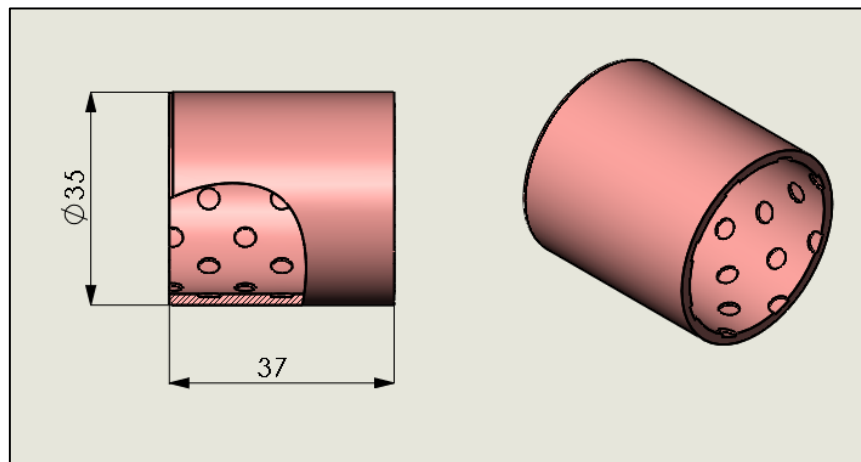
61200B – Bush Anchor Pin
