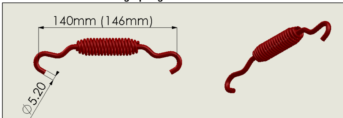
61141 – Brake Shoe Retaining Spring
