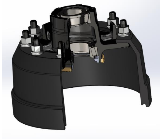
71001 – Single Wheel Stud Hub and Drum Assembly 71001W – 71001 with 1 x 100 tooth pole wheel 61789
