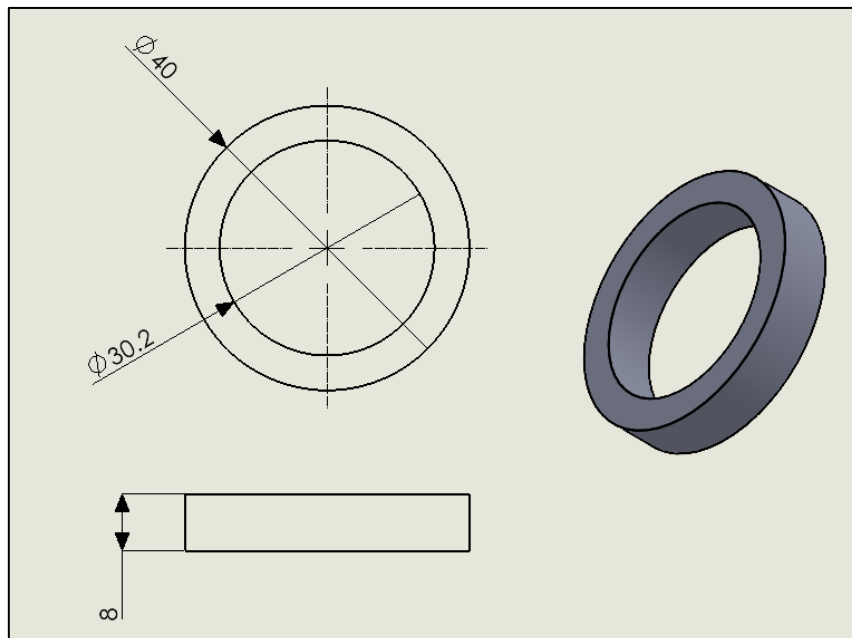
Ram spacer for centre mount - 37242
