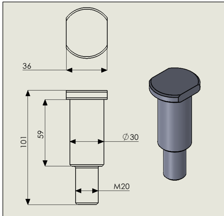
Ram pin for Knuckle bracket 37236
