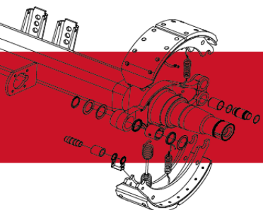
860 "A" Series – No grease nipple in the track rod bolt and steer angle limiting bolt threaded into the beam knuckle.
