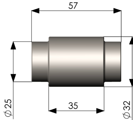
61171 – Anchor pin
