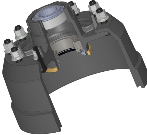
71001 – Single Wheel Stud Hub and Drum Assembly 71001W – 71001 with 1 x 100 tooth pole wheel 61789
